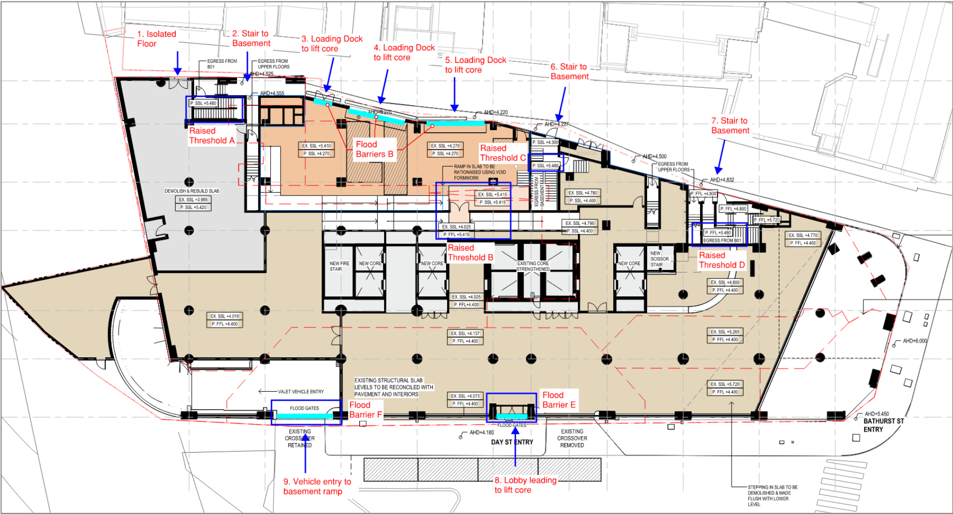
Figure 21: Flood Planning Levels Compliance
