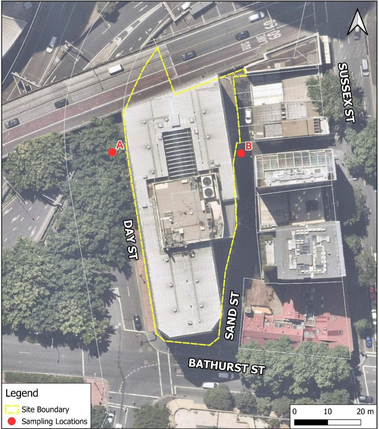
Figure 11: Sampling Points for Comparison of Flood Results
